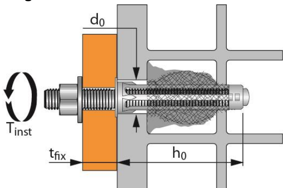
Figure A1: Perforated sleeve in hollow masonry
